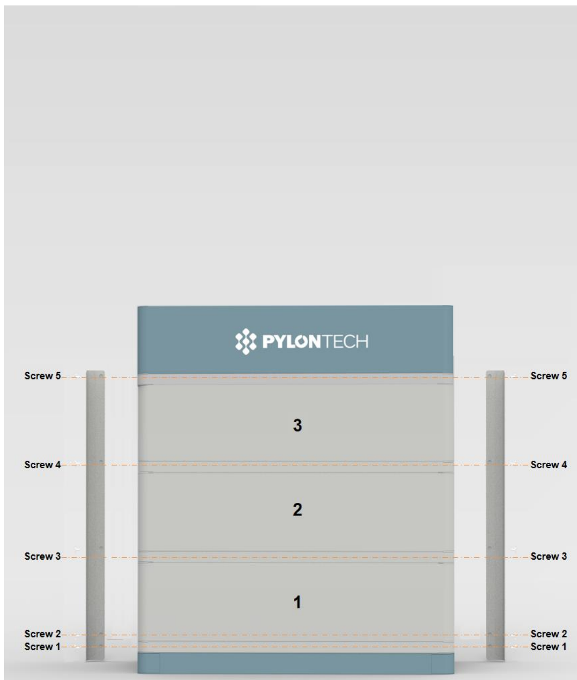
3.4.8 Locking of the control Module's fix screw of left and right side
